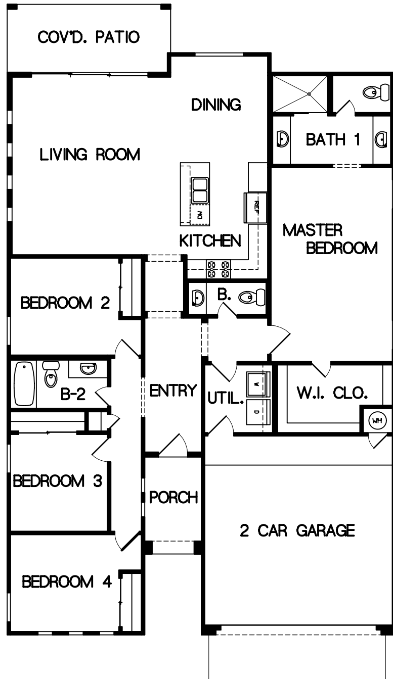
FLOOR PLAN
