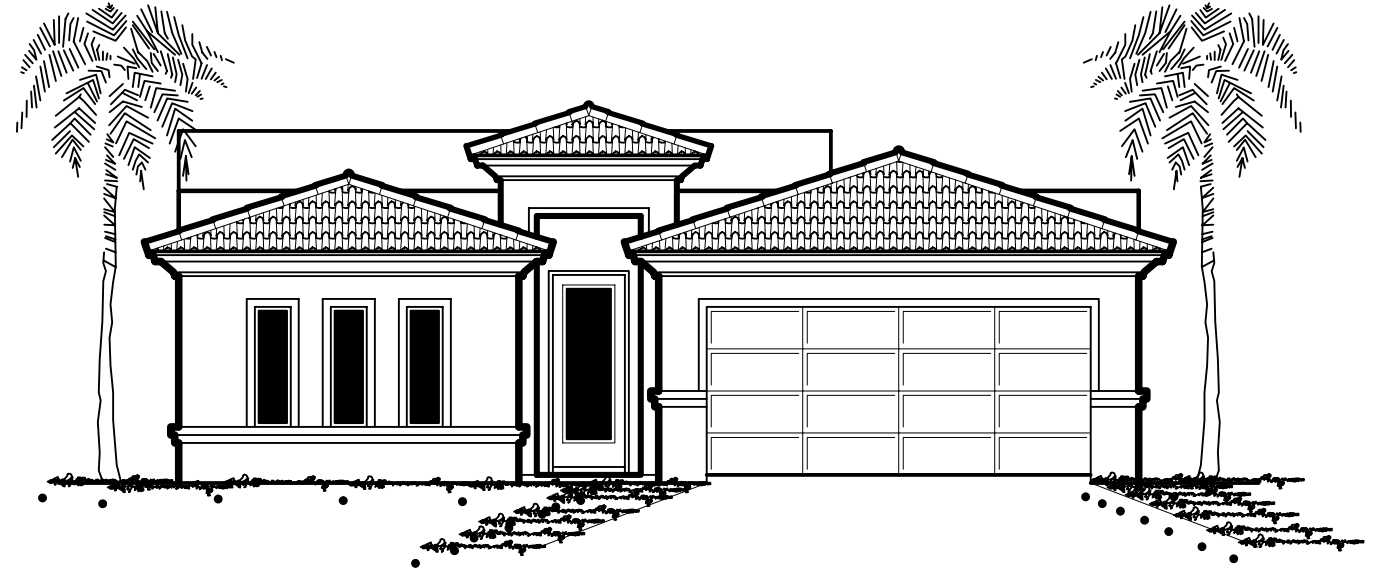
FRONT ELEVATION
